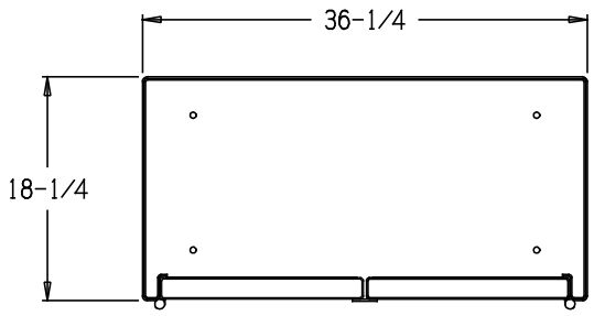
TOP SECTION VIEW
