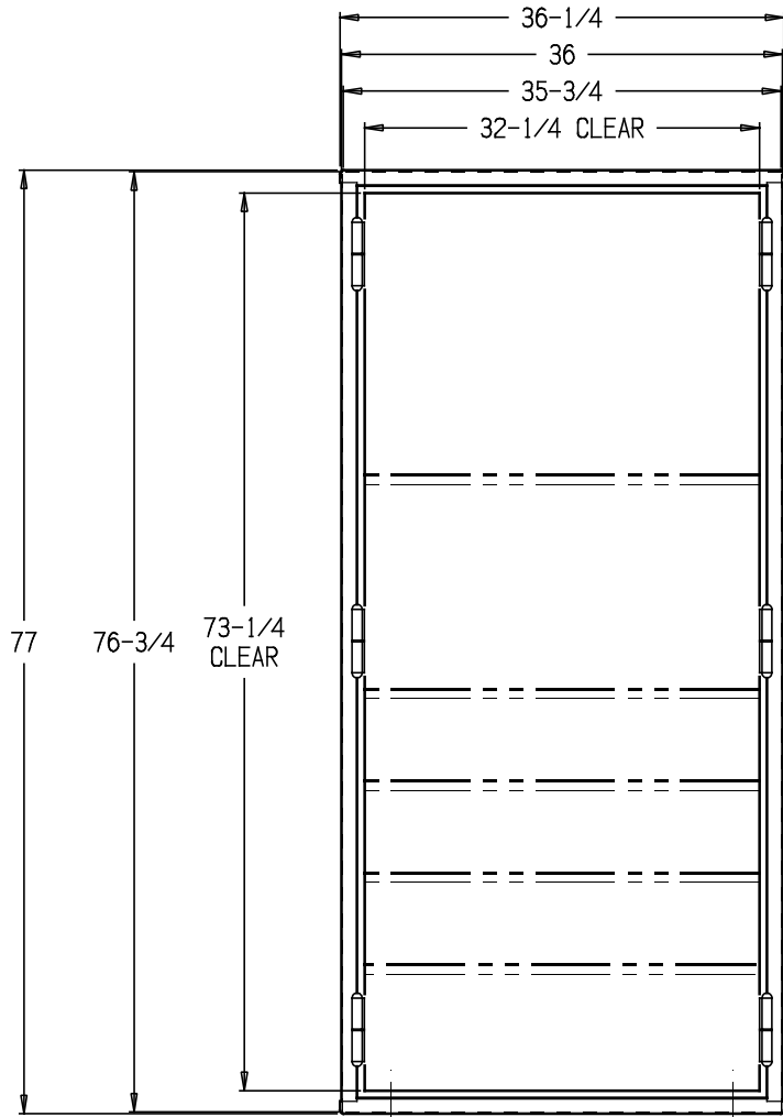
FRONT VIEW (SHOWN WITHOUT DOORS)
